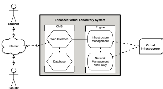
Figure 4: Project Architecture
