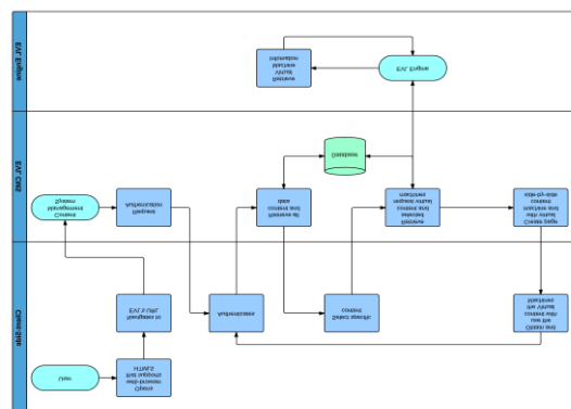
Figure 3: Conceptual Model
